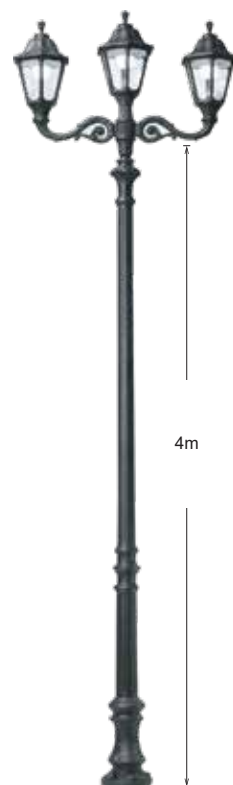
Lantern: Rut 2L+1 System Bracket: Adam Post: Karmel Watts: 3 x 6W-11W Lamp: E27
