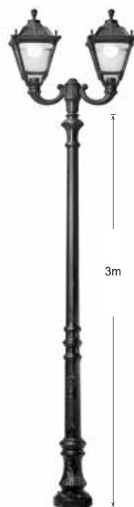
Lantern: Tobia 2L System Bracket: Ofir Post: Karmel Watts: 2x 15W-30W Lamp: E27
